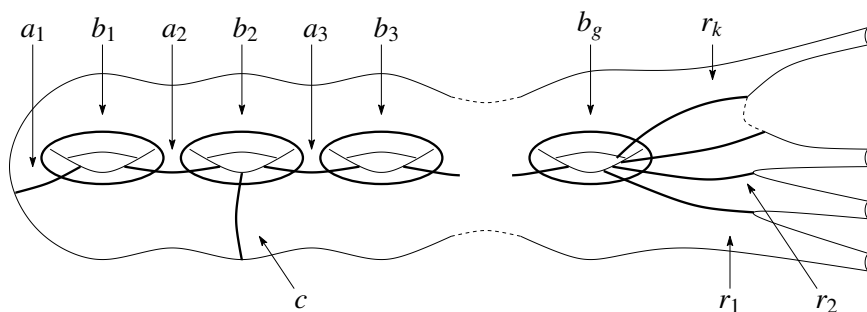
Figure 1: Dehn twists along the curves a_i, b_i, c and r_i generate \text{Map}(X) .
